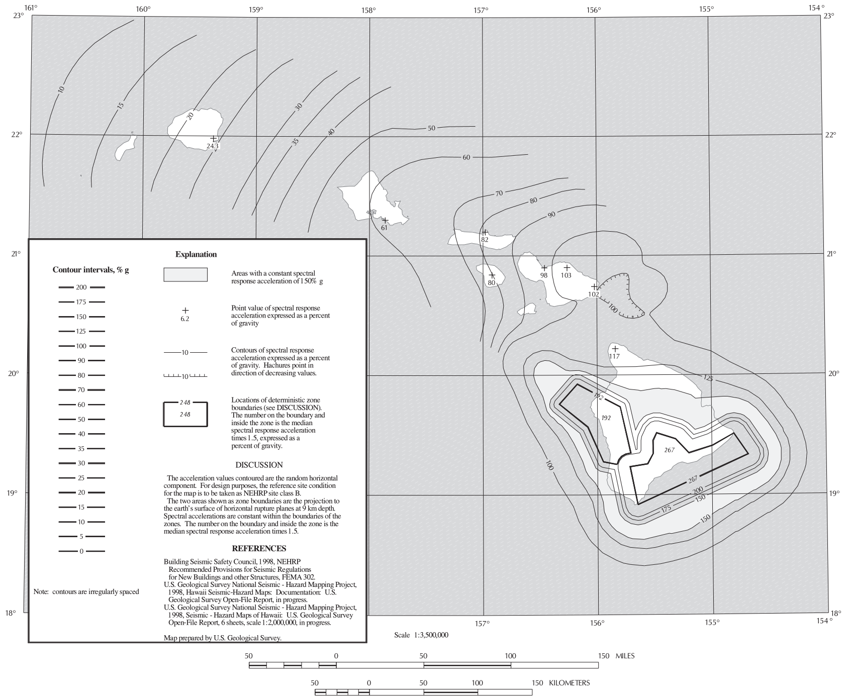
FIGURE 9.4.1.1 (h-1) MAXIMUM CONSIDERED EARTHQUAKE GROUND MOTION FOR HAWAII OF 0.2 SEC SPECTRAL RESPONSE ACCELERATION (5% OF CRITICAL DAMPING), SITE CLASS B
