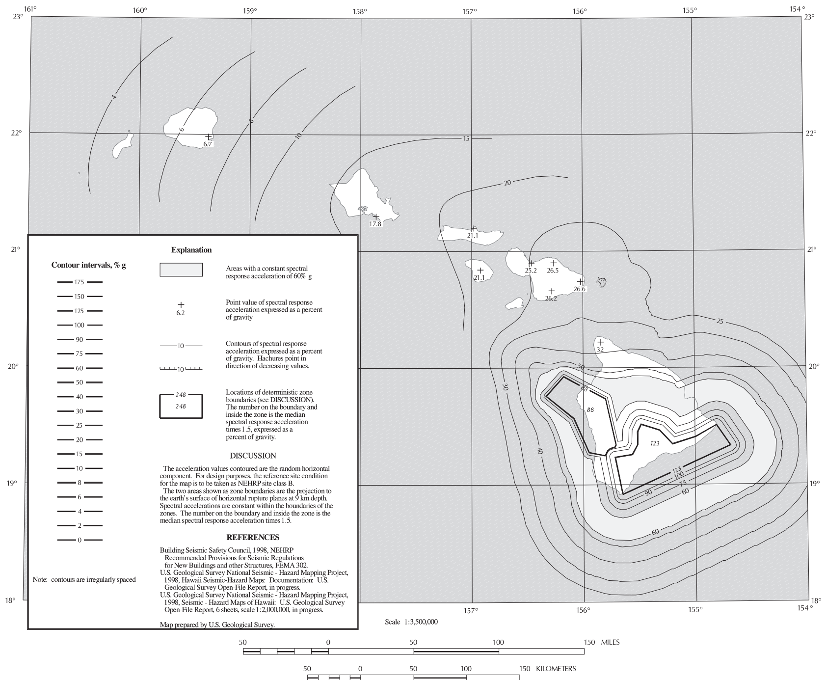
FIGURE 9.4.1.1 (h-2) MAXIMUM CONSIDERED EARTHQUAKE GROUND MOTION FOR HAWAII OF 1.0 SEC SPECTRAL RESPONSE ACCELERATION (5% OF CRITICAL DAMPING), SITE CLASS B
