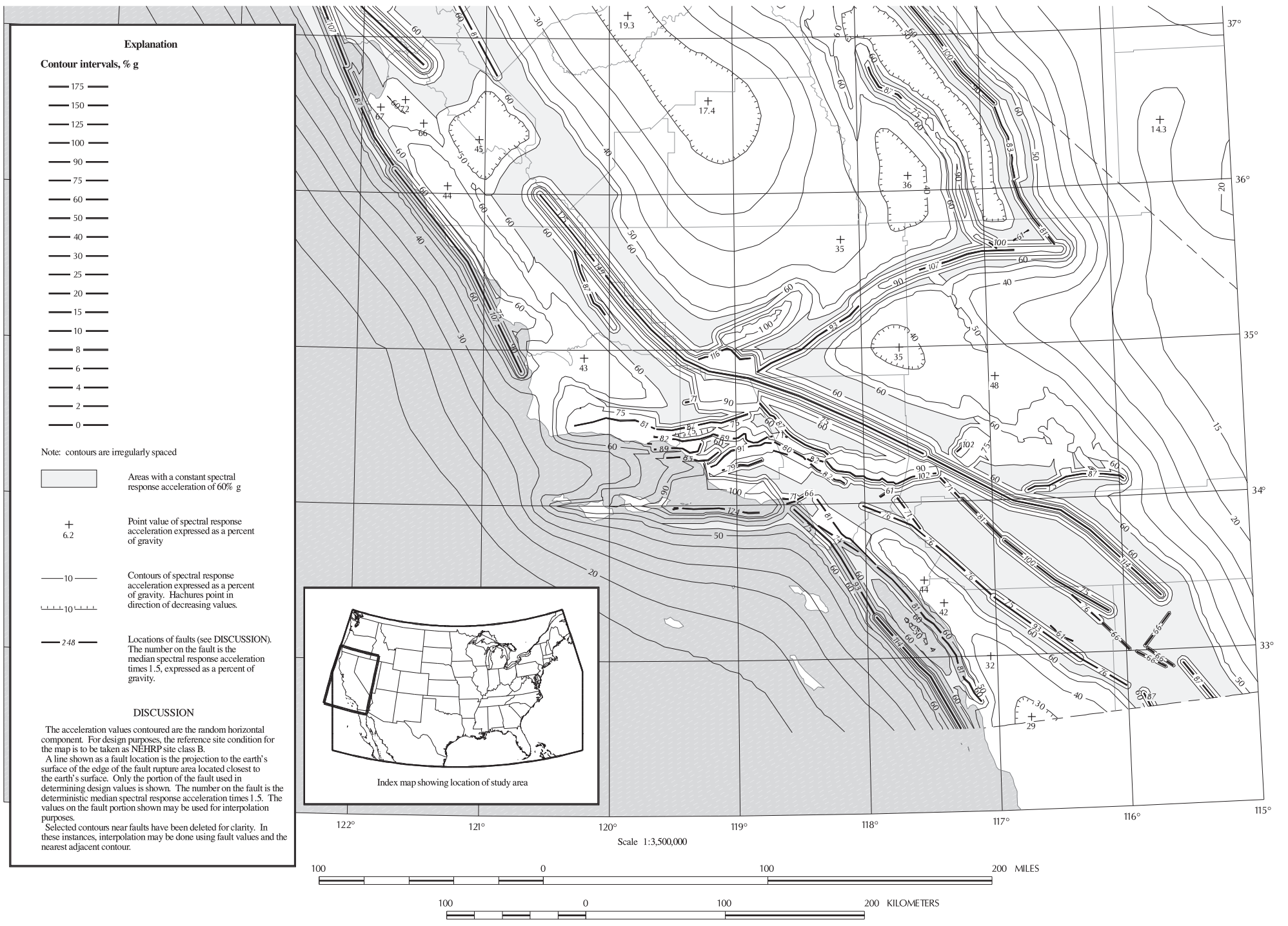
FIGURE 9.4.1.1 (d) (continued) MAXIMUM CONSIDERED EARTHQUAKE GROUND MOTION FOR REGION 1 OF 1.0 SEC SPECTRAL RESPONSE ACCELERATION (5% OF CRITICAL DAMPING), SITE CLASS B
