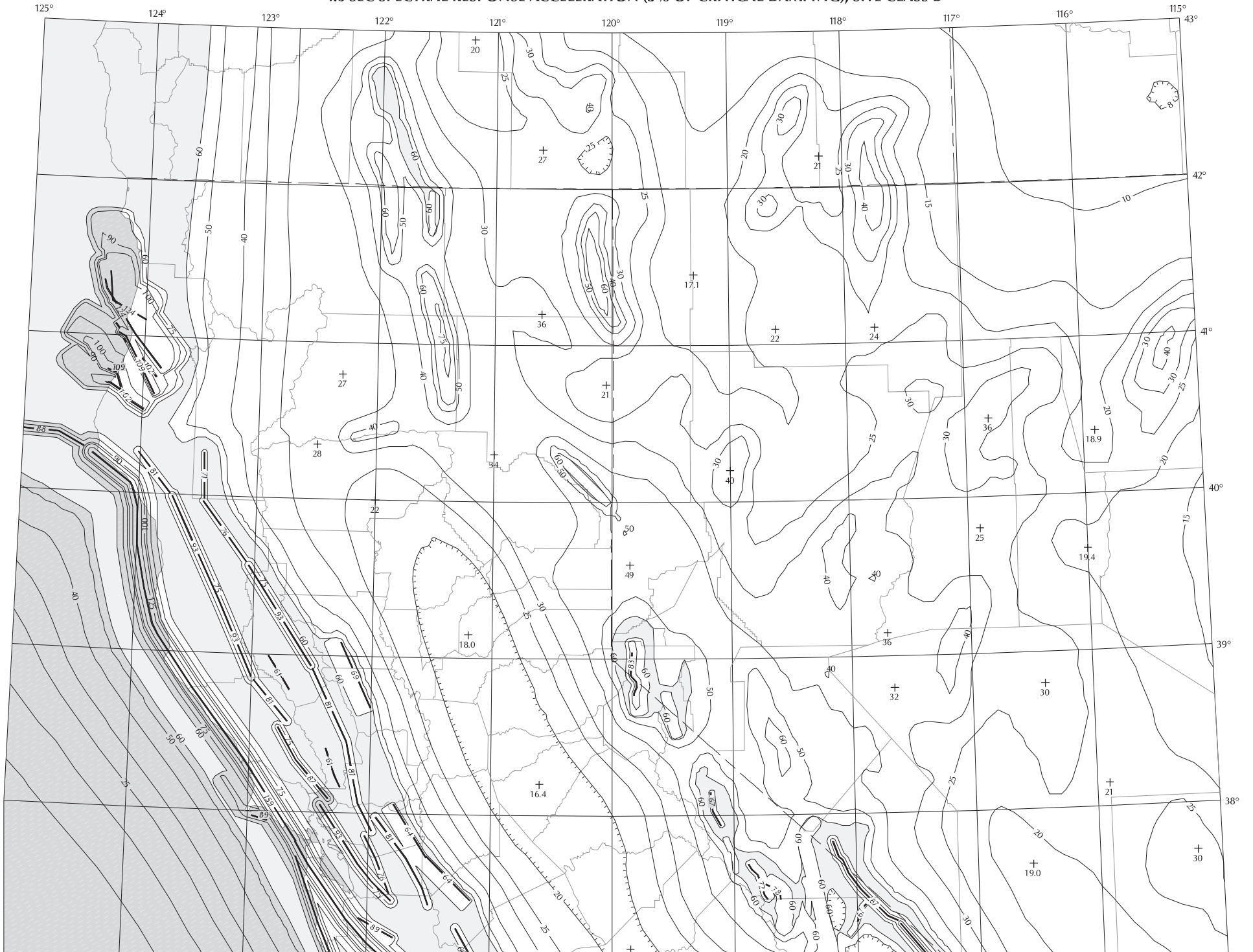
FIGURE 9.4.1.1 (d) MAXIMUM CONSIDERED EARTHQUAKE GROUND MOTION FOR REGION 1 OF 1.0 SEC SPECTRAL RESPONSE ACCELERATION (5% OF CRITICAL DAMPING), SITE CLASS B
